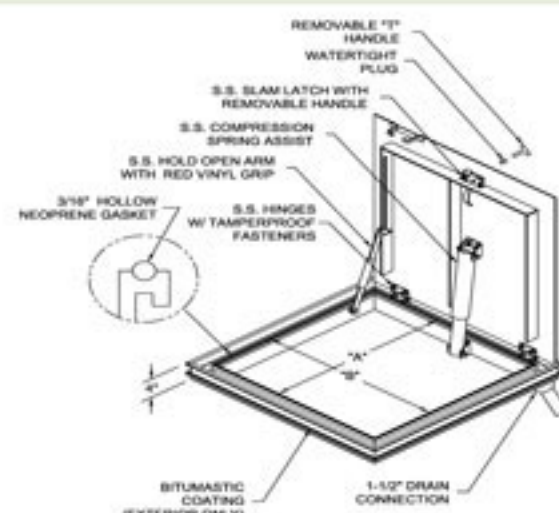
View of KFD-SD Water Tight Door
